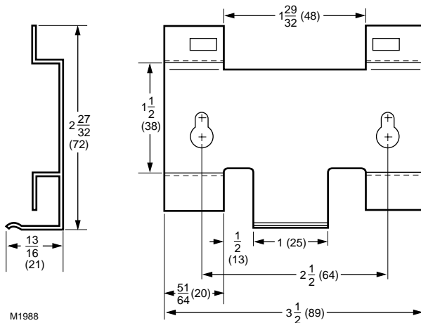
Fig. 1. 203765 Remote Mounting Bracket dimensions in in. (mm).
